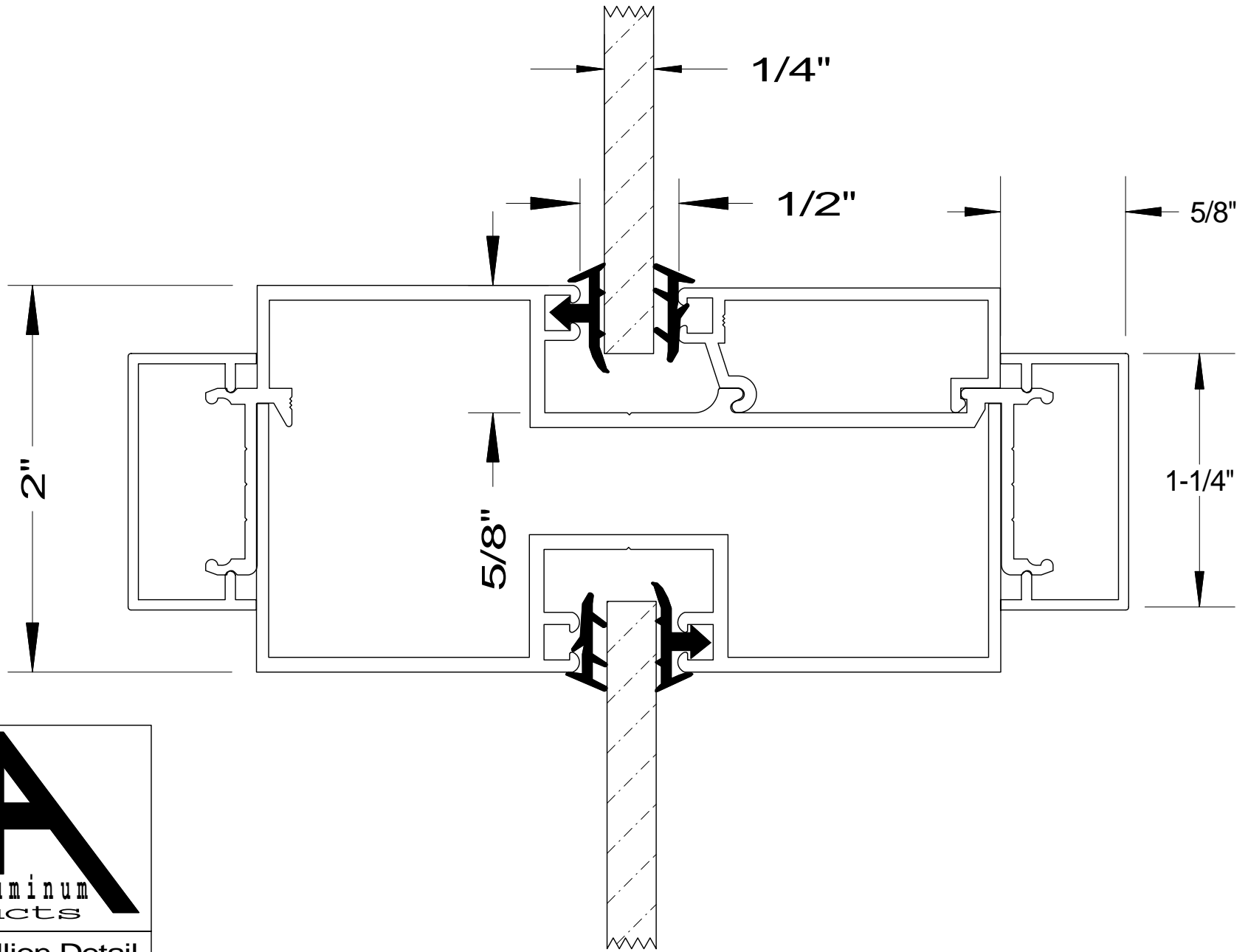
Horizontal Mullion Detail with 125 Trim
